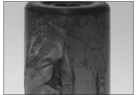
Fig. 28. Overloading on this cylindrical roller bearing caused roller surfaces to fracture.
