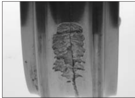
Fig. 27. This ball bearing inner ring depicts fatigue spalling from high loads. The fracture is a secondary damage mode.
